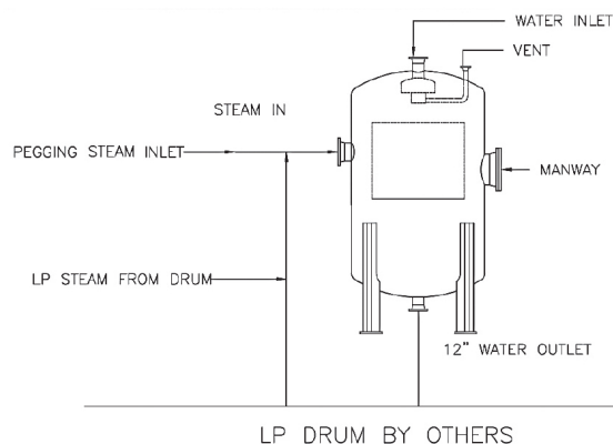
OUTLINE – VERTICAL DEAERATOR
